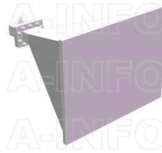
LB-229-20-C-NFSPO Standard Gain Horn Antenna 3.3-4.9GHz 20dB Gain N Type Female
